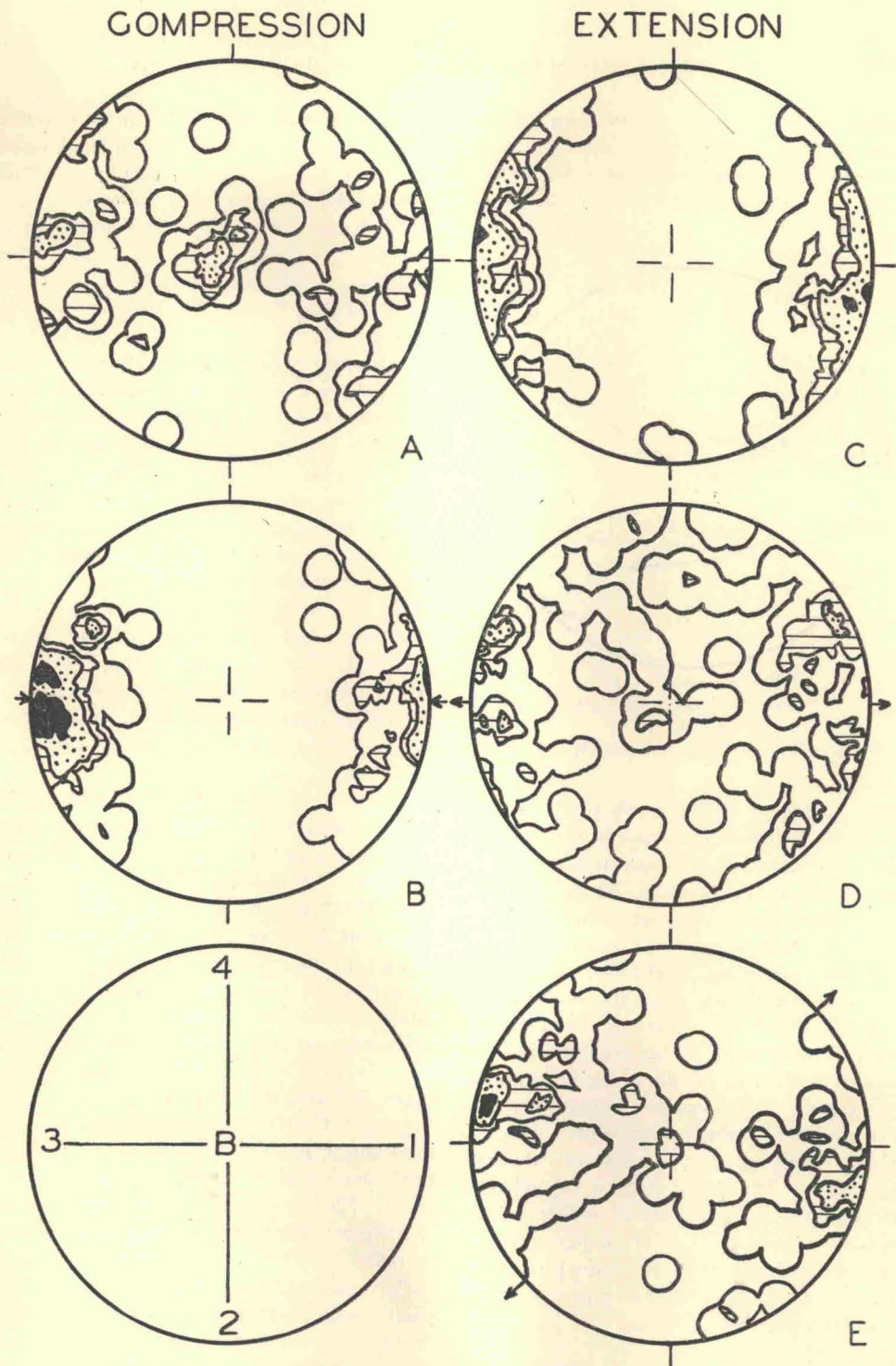
FIGURE 7.—ORIENTATION DIAGRAMS FOR c AXES OF CALCITE IN DEFORMED YULE MARBLE 100 grains per diagram. Contours, 1, 3, 5, 10%, per 1% area. Diagrams oriented (cf. bottom left) with trace of foliation plane (1 and 3) parallel to N-S diameters.
